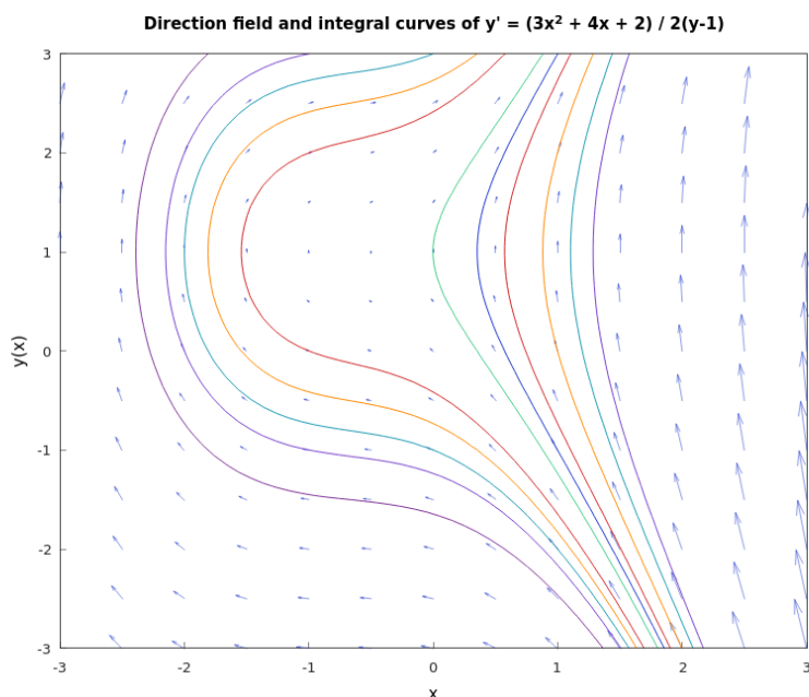
Figure 5.27: The direction field and integral curves of \frac{dy}{dx} = \frac{3x^2+4x+2}{2(y-1)} (Hamzstplot/Examples with Makefile/Plot First Order Differential Equation Direction Field and Solutions Curves for Separable Equations Example 2/main.cpp).
