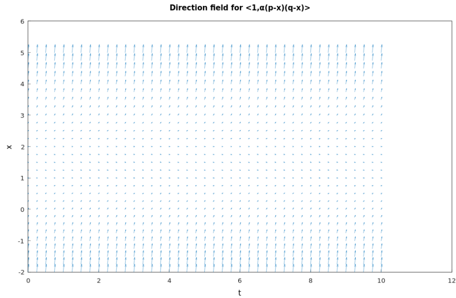
Figure 5.55: The direction field for \langle 1, \alpha(p-x)(q-x) \rangle with \alpha = 1 , p = 1 , and q = 2 (Hamzstplot/Examples with Makefile/Plot Direction Fields for Chemical Reactions Problem 28a/main.cpp).
