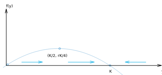
Figure 5.28: The equilibrium solution f(y) = 0 or r(1 - y/K)y = 0 to visualize other solutions of Eq. (4.53) ( Hamzstplot/Examples with Makefile/Plot 2D Equilibrium Solution for Logistic Growth/main.cpp ).
