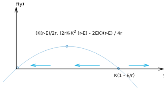
Figure 5.35: The equilibrium points and the stability analysis for \frac{dy}{dt} = f(y) = \left(y - K\left(1 - \frac{E}{r}\right)\right)y (Hamzstplot/Examples with Makefile/Plot 2D Equilibrium Solution for Schaefer Model/main.cpp).
