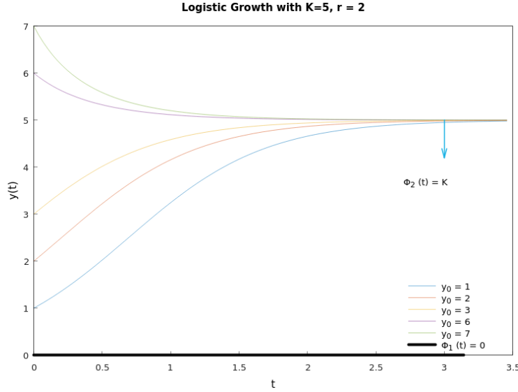
Figure 5.29: The solution curves for y(t) = \frac{y_0 K}{y_0 + (K - y_0)e^{-rt}} to visualize all possible solutions of Eq. (4.53) with different y_0 (Hamzstplot/Examples with Makefile/Plot 2D Solution Curves for Logistic Growth/main.cpp).
